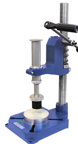
Fig. 3: Testing the chalking rate using a stand
